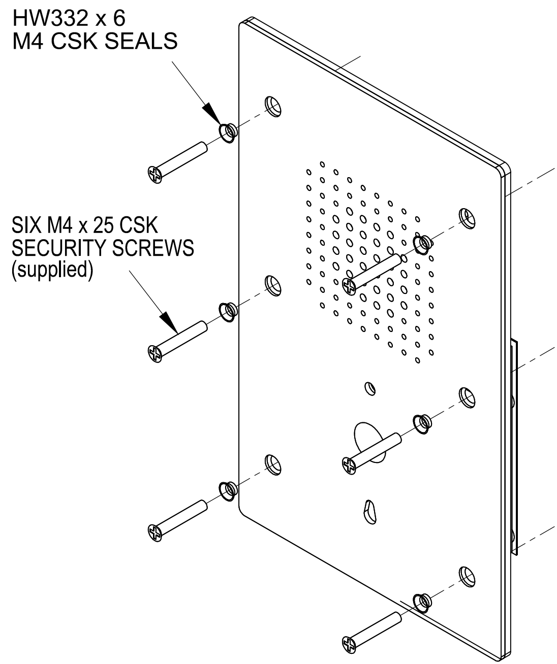
VIEW SHOWING PANEL FIXINGS
