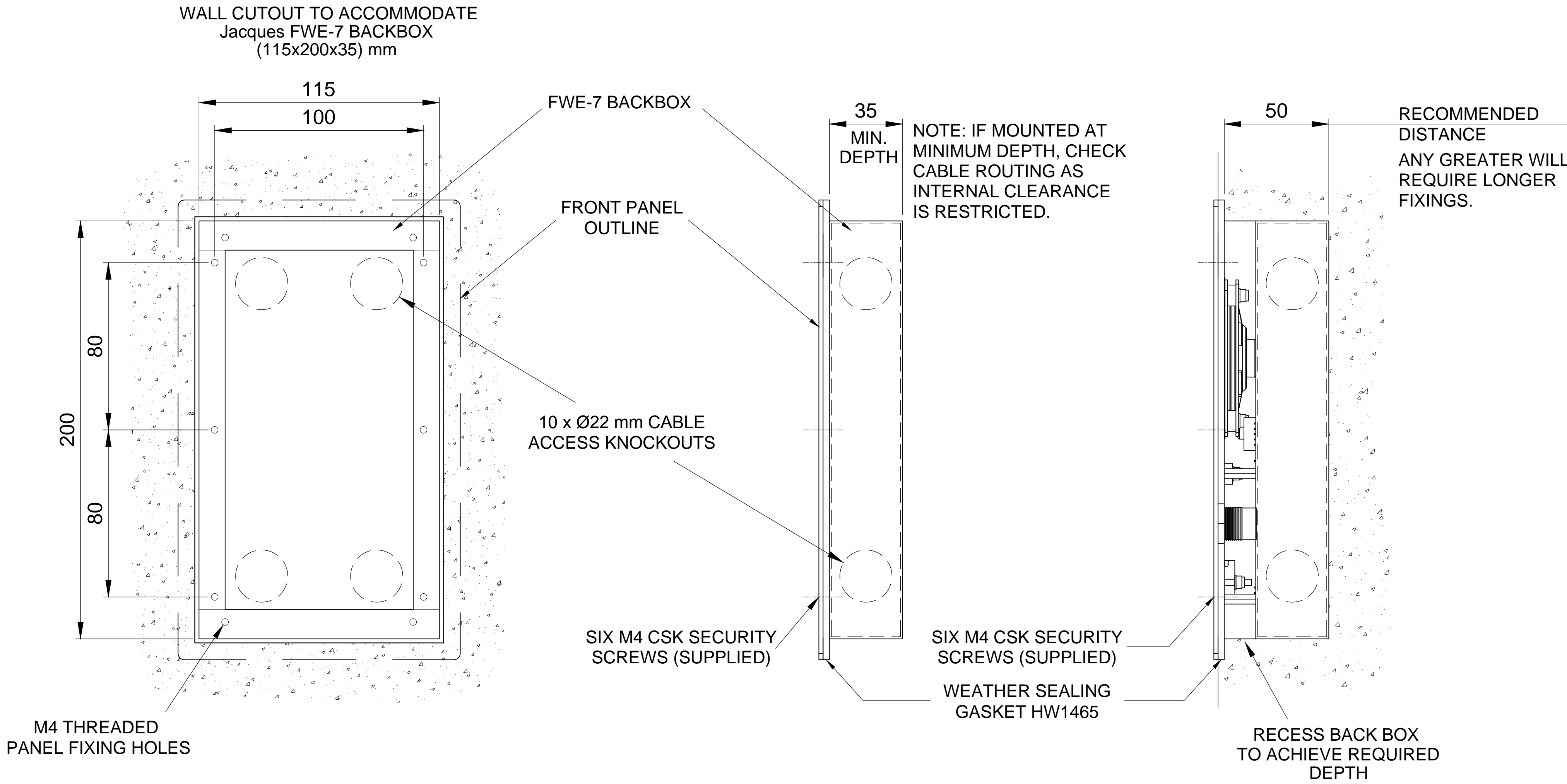
FLUSH WALL MOUNTING USING FWE-7 BACKBOX
