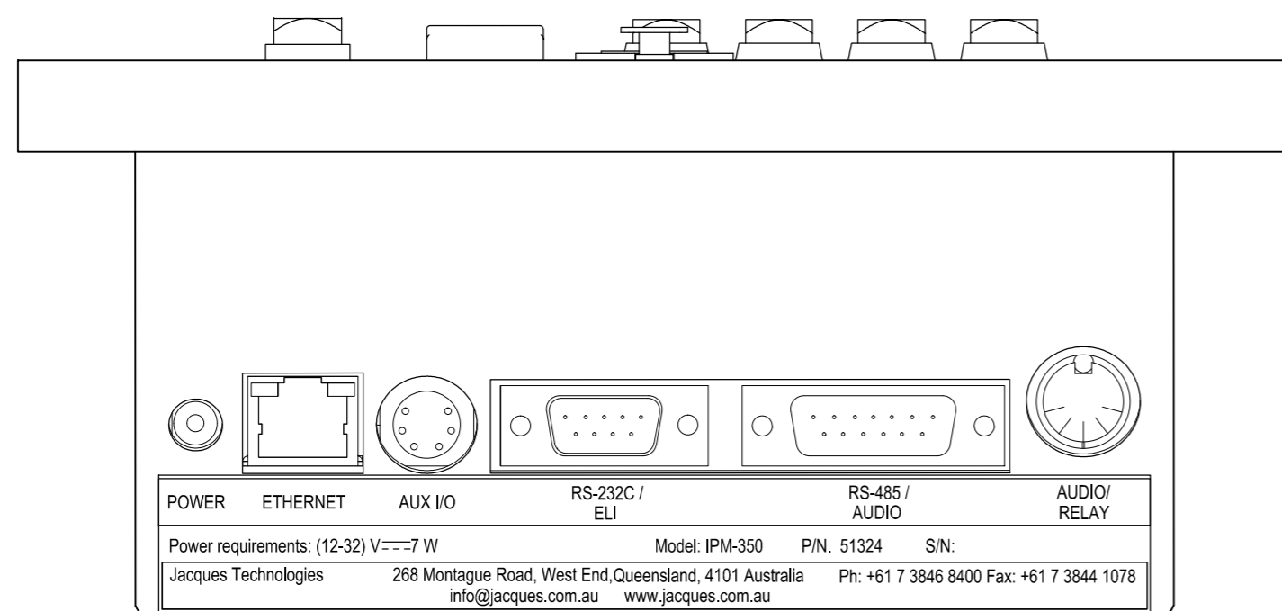
VIEW SHOWING CONNECTORS
