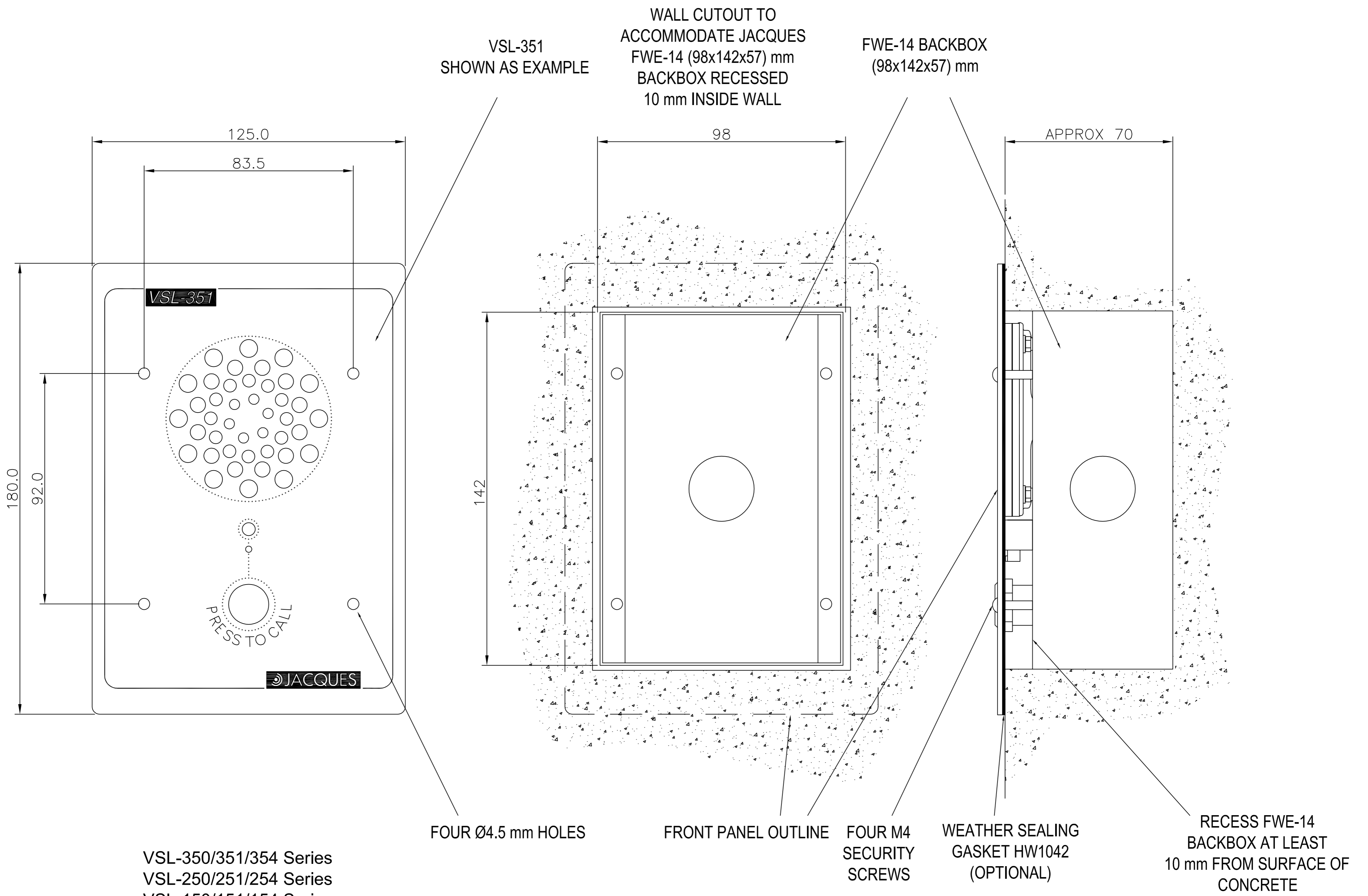
FLUSH WALL MOUNT USING FWE-14 BACKBOX
