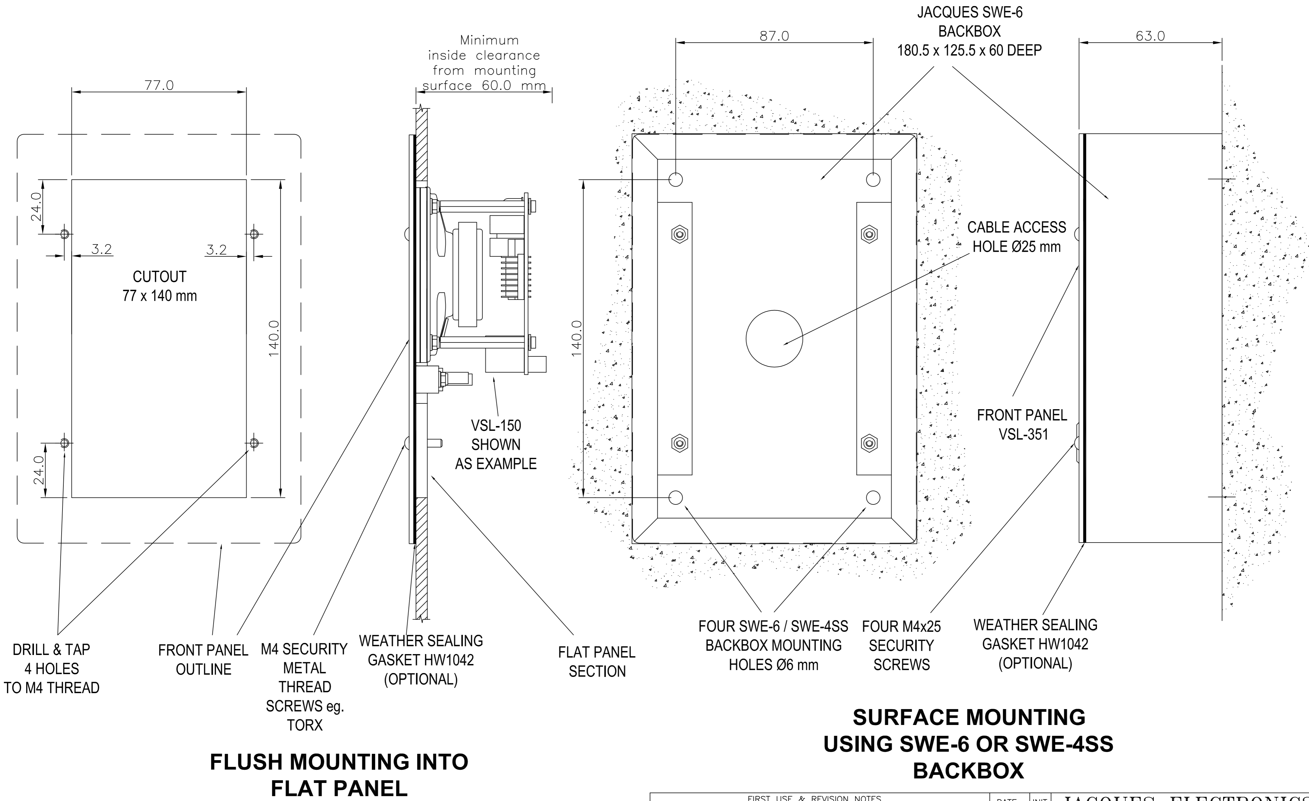
VSL-350/351/354 Series VSL-250/251/254 Series VSL-150/151/154 Series Slave Intercom Station FRONT PANEL LAYOUT AND DIMENSIONS
